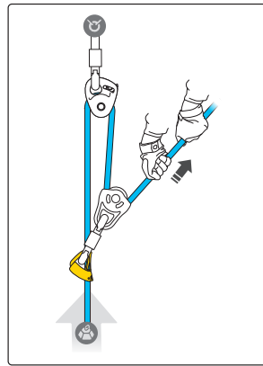
Hauling gear
