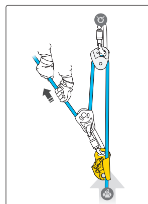
Pulley system with a BASIC ascender
