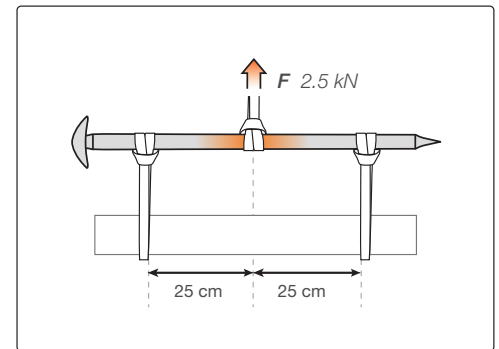
Pull test
