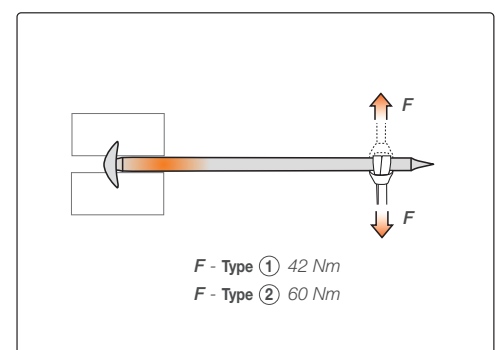
Levering test
